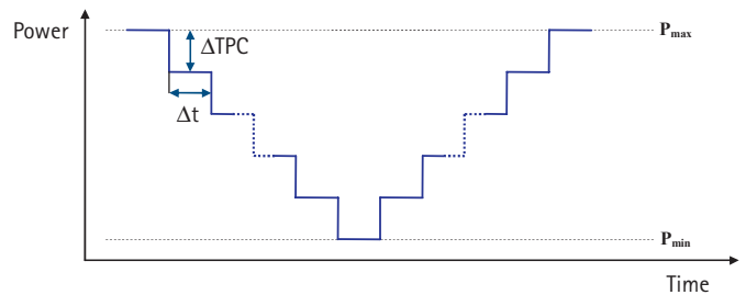
Figure 3: Inner Loop Power Control
