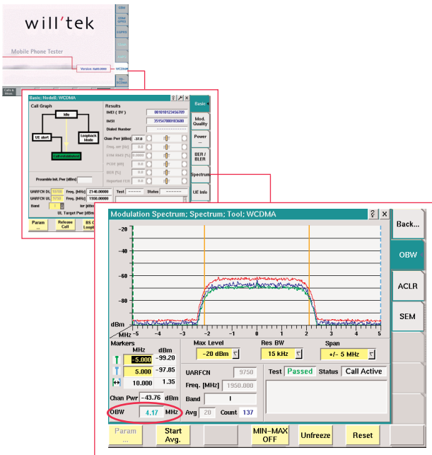
Figure 4: Occupied Bandwidth
