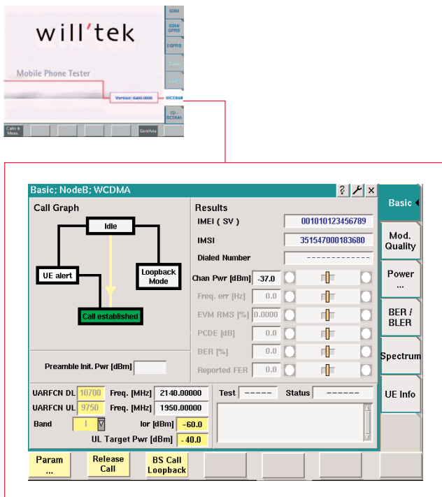
Figure 1: WCDMA Basic Menu – call established
