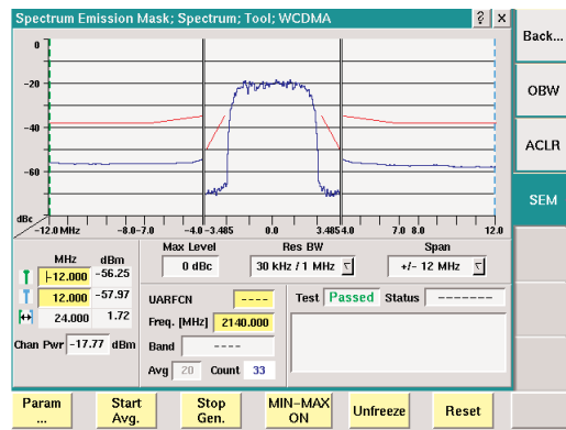
Figure 6: Spectrum Emission Mask (SEM)
