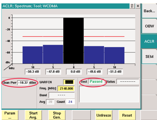
Figure 5: Adjacent Channel Leakage Power Ratio
